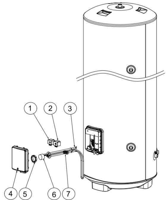
Diagram 1 – Cylinder Detail
