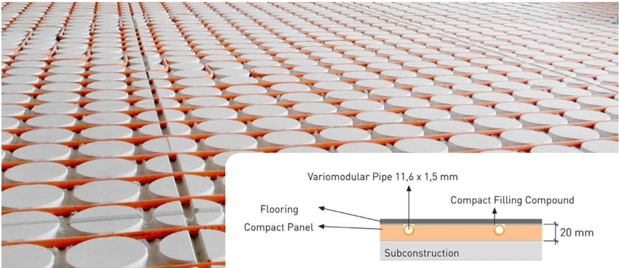
Cross-section of Variotherm system
