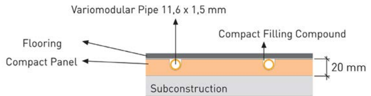
Cross-section of Variotherm system
